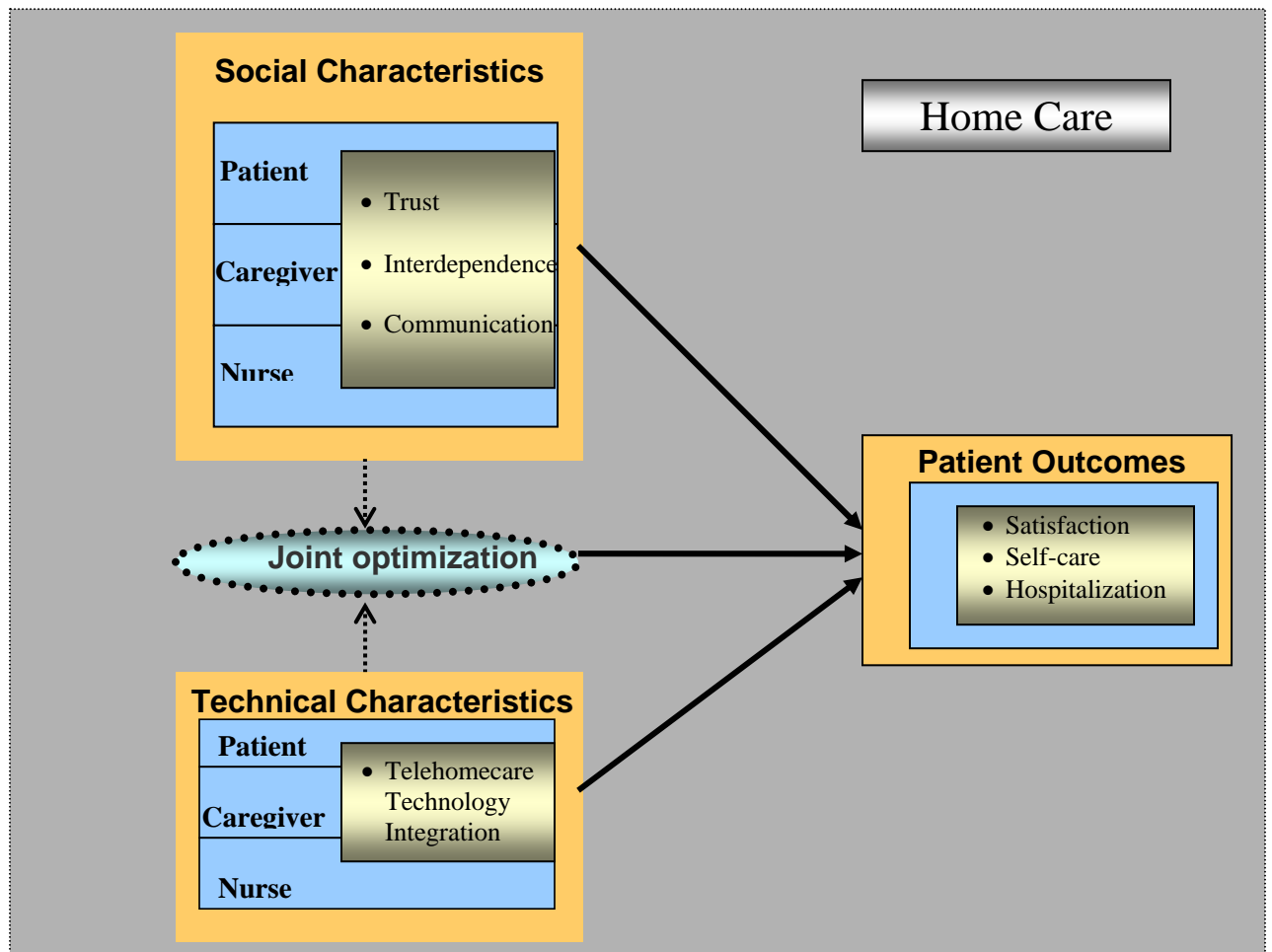
FIGURE 2. Research Model
